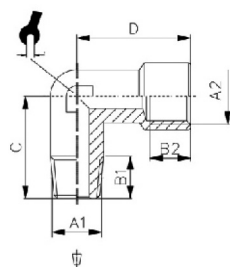
MALE - FEMALE ELBOW / L MALE - FEMELLE / L MASCHIO - FEMMINA
