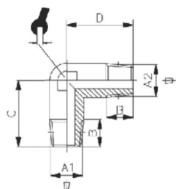
MALE ELBOW / L MALE / L MASCHIO
