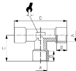
FEMALE TEE / T FEMELLE / T FEMMINA
