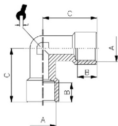
FEMALE ELBOW / L FEMELLE / L FEMMINA
